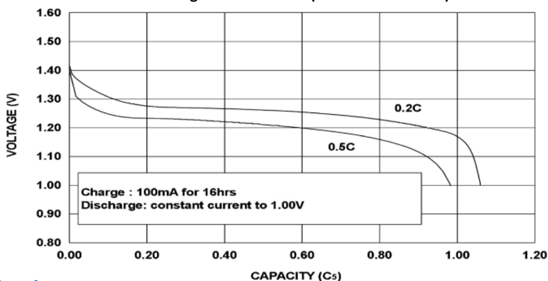
Discharge characteristics (load 0.2C – 200 mA):
