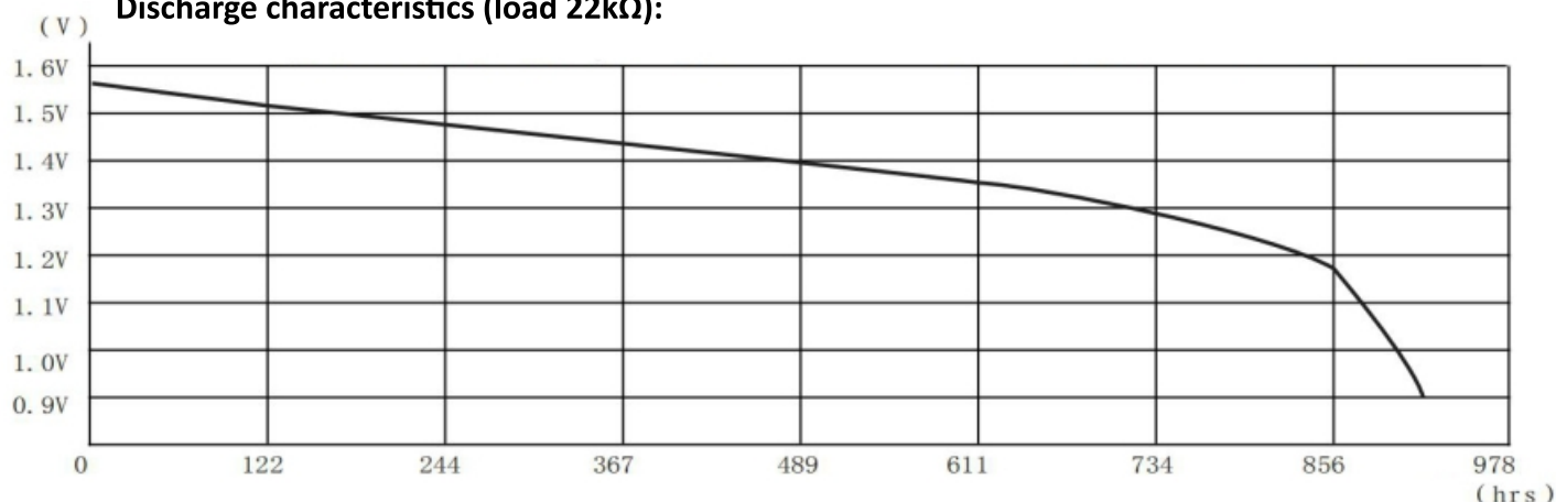
Discharge characteristics (load 22k \Omega ):
