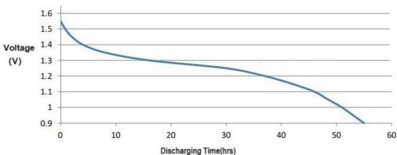
Discharge characteristics (load 22k \Omega ):
