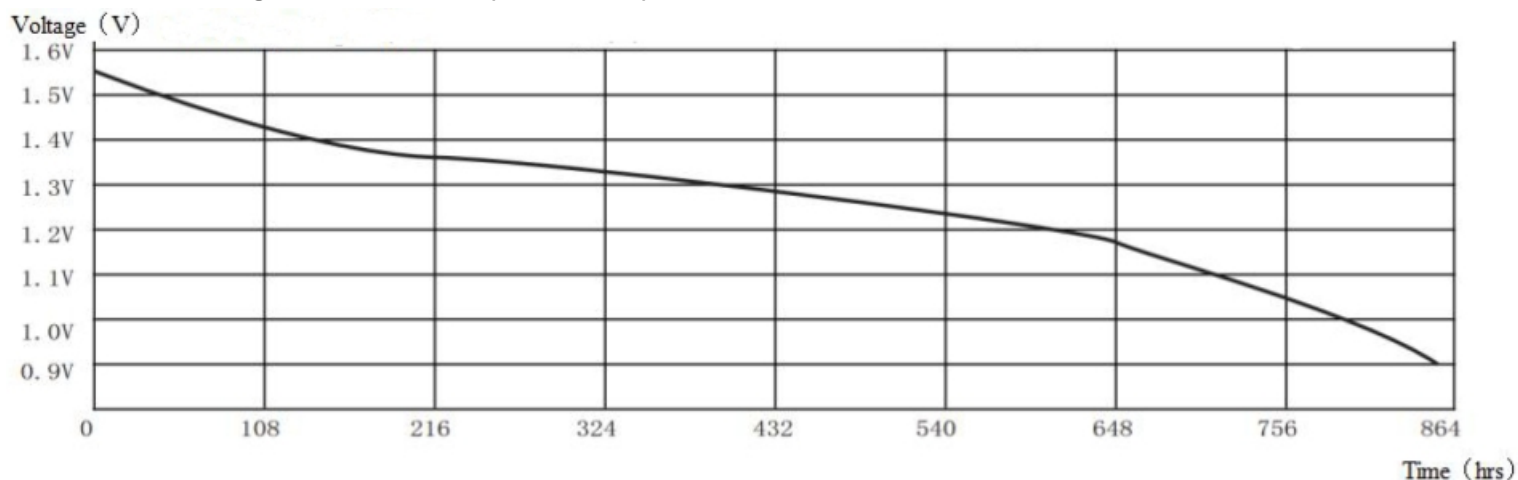
Discharge characteristics (load 6.8kΩ):
