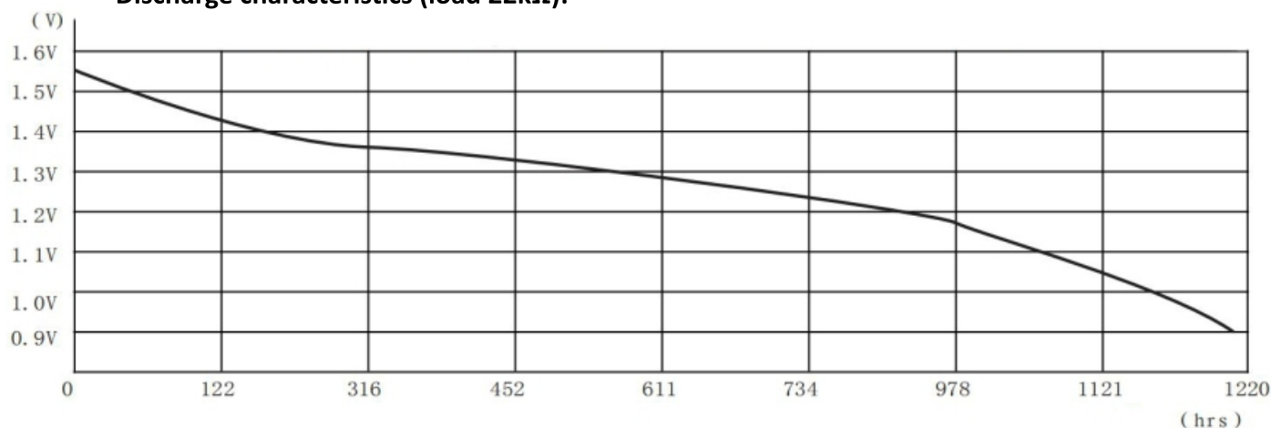
Discharge characteristics (load 22k \Omega ):
