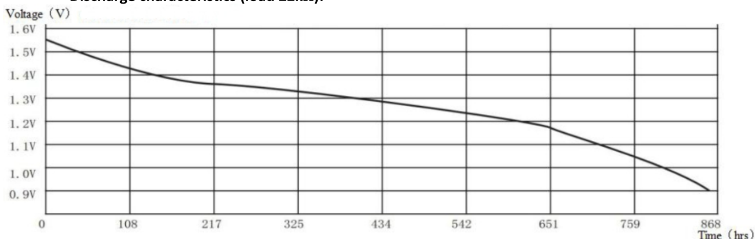
Discharge characteristics (load 22k \Omega ):
