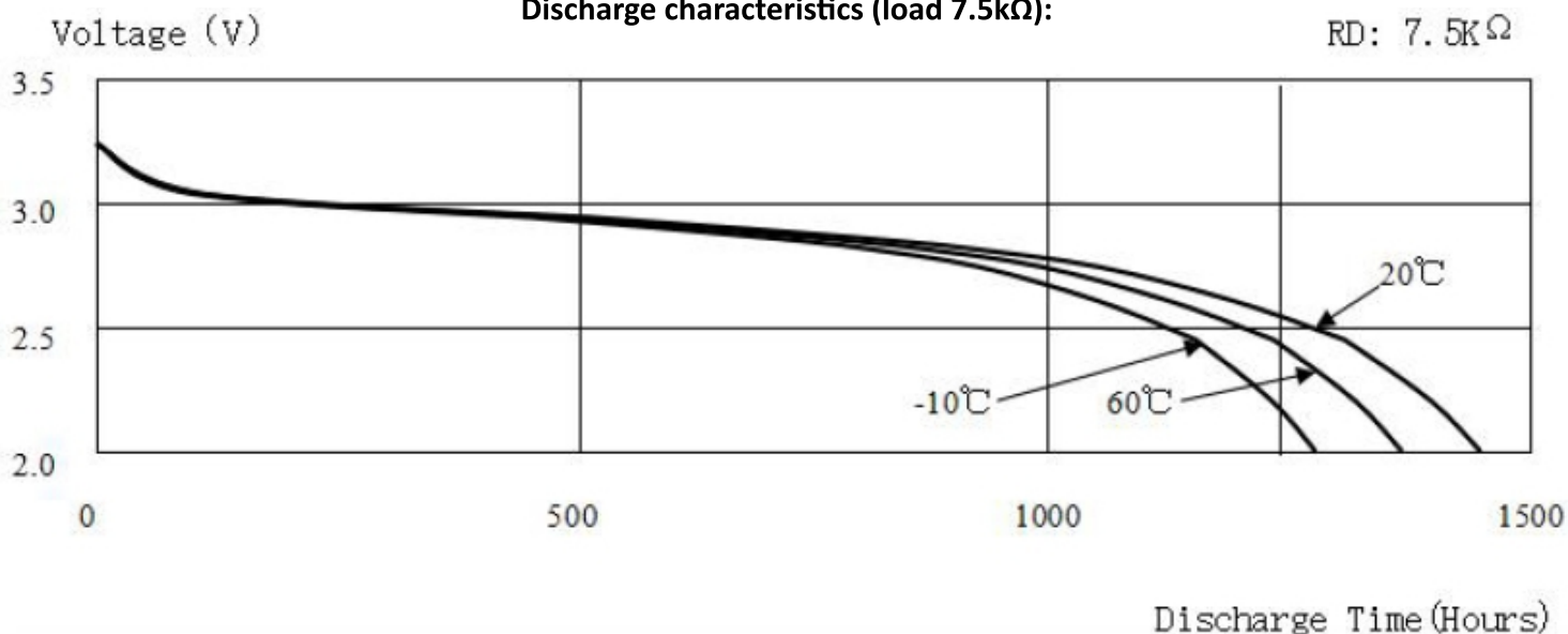
Discharge characteristics (load 7.5kΩ):
